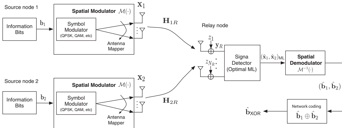
FIGURE 2. Transmission and reception in the MA phase.
